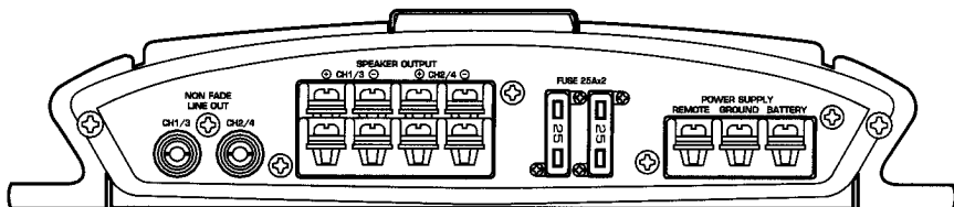
Figure 3. Rear panel layout of the Clarion APA4203 amplifier.
